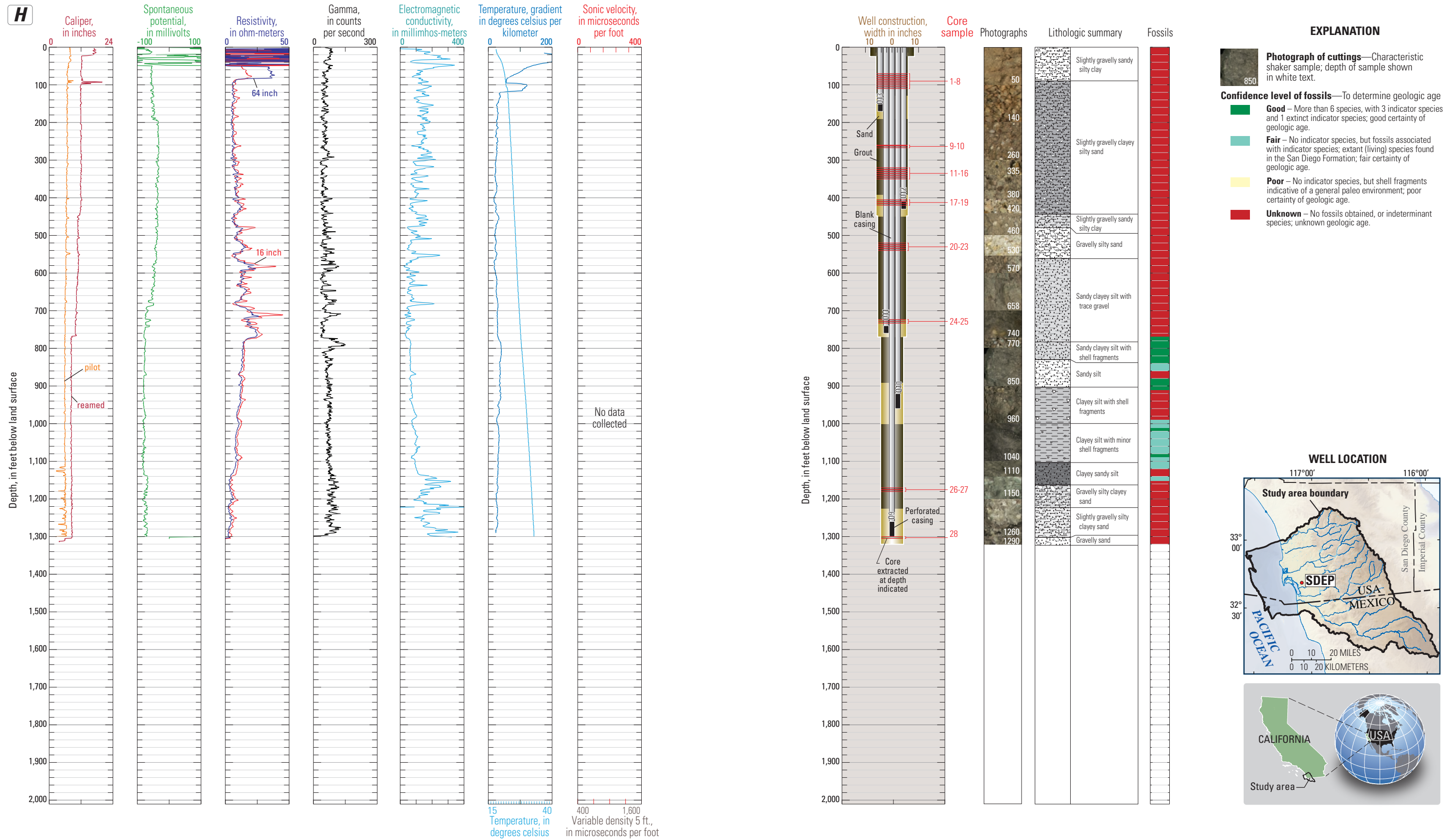
Figure 19H. Well-construction diagrams, generalized lithologic descriptions, and geophysical-log data for caliper, spontaneous potential, resistivity, natural gamma, electromagnetic conductivity, temperature, and sonic logs collected from 16 USGS multiple-depth, monitoring-well sites in San Diego County, California, 1995, 2003–2017: (A) SDCD; (B) SDSY; (C) SDLH; (D) SDAQ; (E) SDCP; (F) SDBP; (G) SDHF; (H) SDEP ; (I) SDNB; (J) SDSW; (K) SDMC; (L) SDLD; (M) SDCC; (N) SDOR; (O) SDOT; and (P) SDBW.—Continued.
